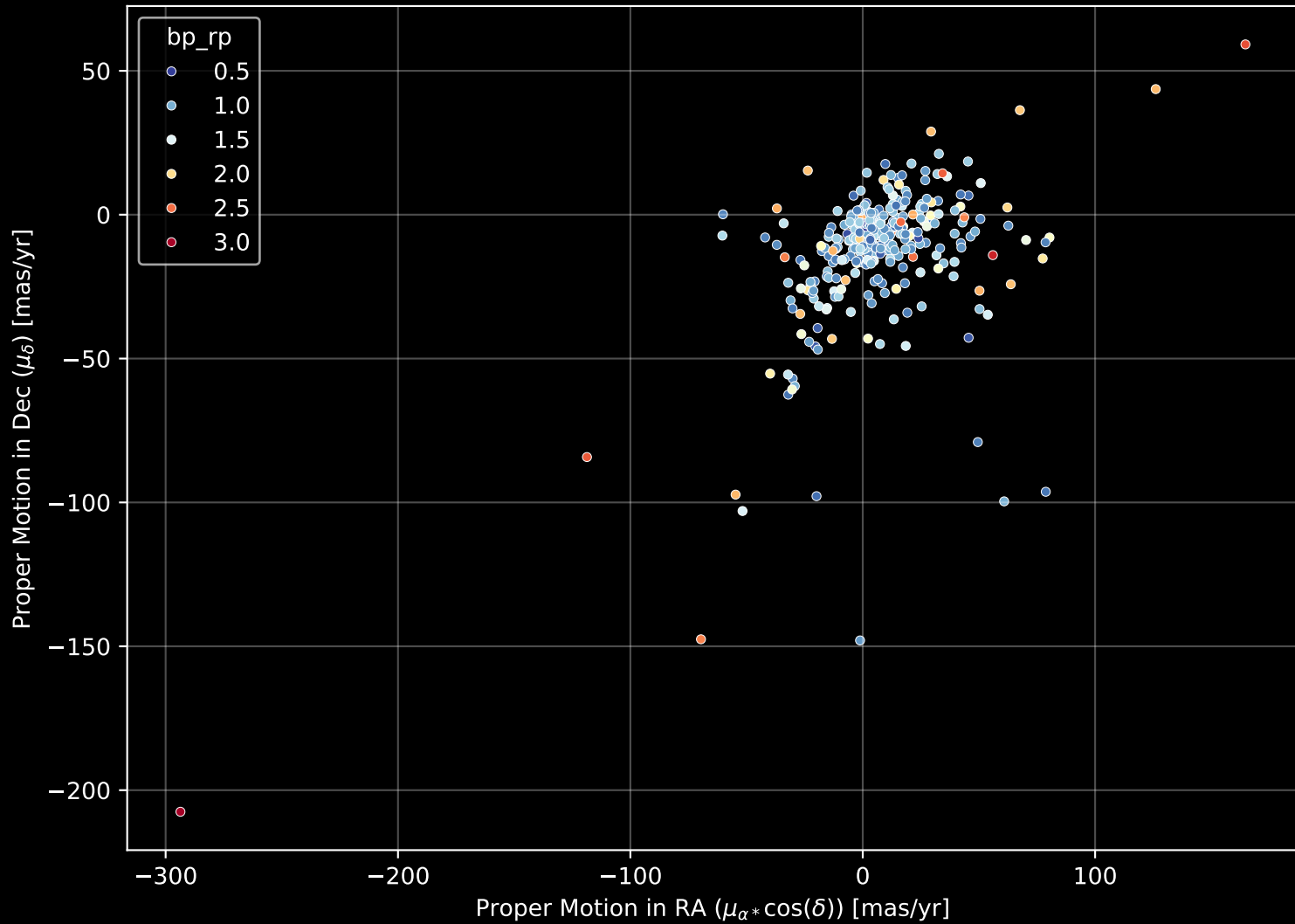
APOGEE DR17 Field: [sgr_tidal10] Proper Motion Diagram (n= 315)
