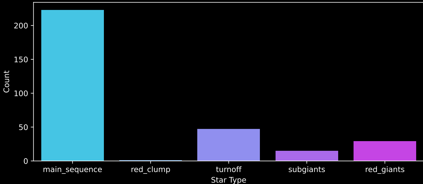
APOGEE DR17 Field: [sgr_tidal10] Count plot of Star Type
