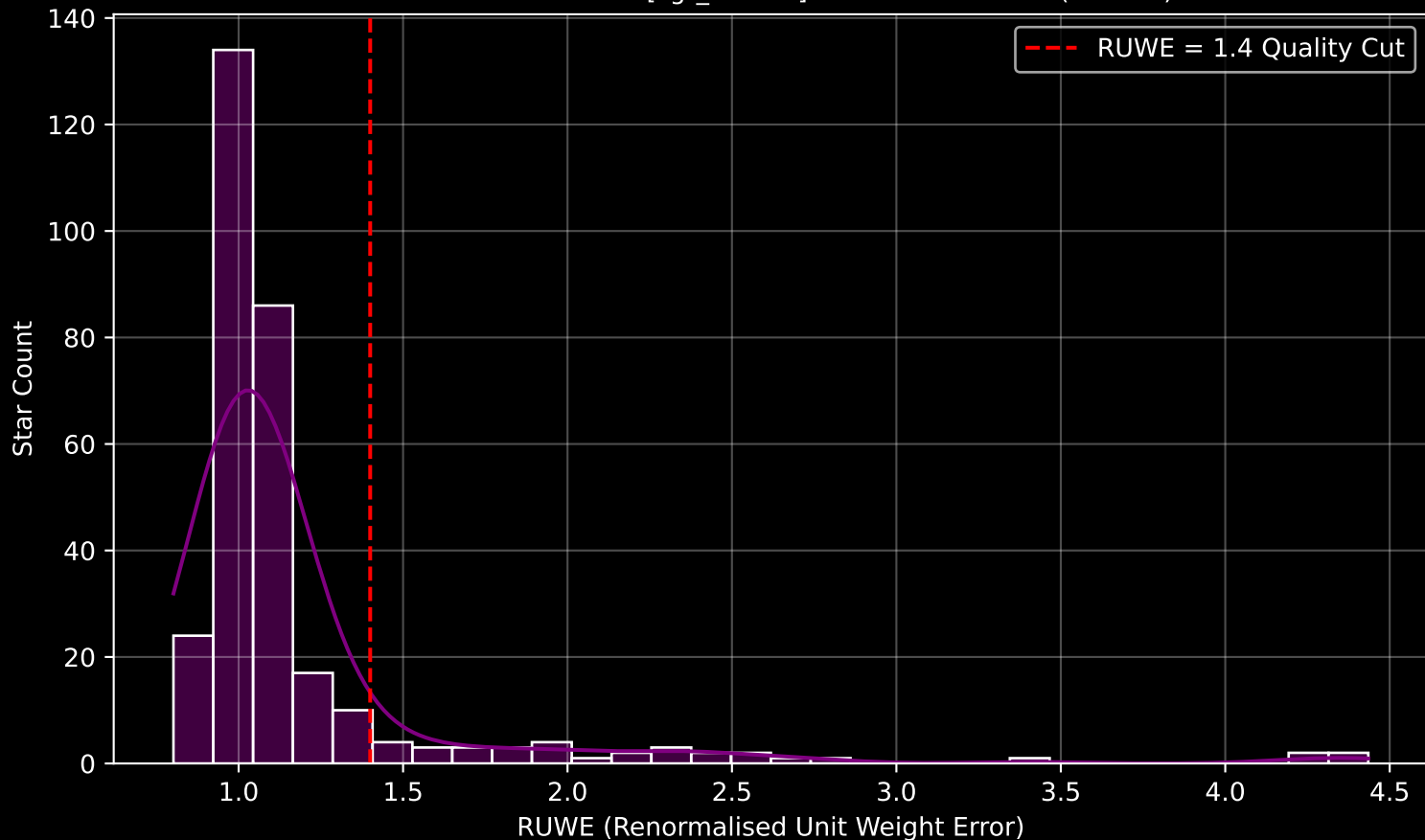
GAPOGEE DR17 Field [sgr_tidal10] RUWE Distribution (n= 305)
