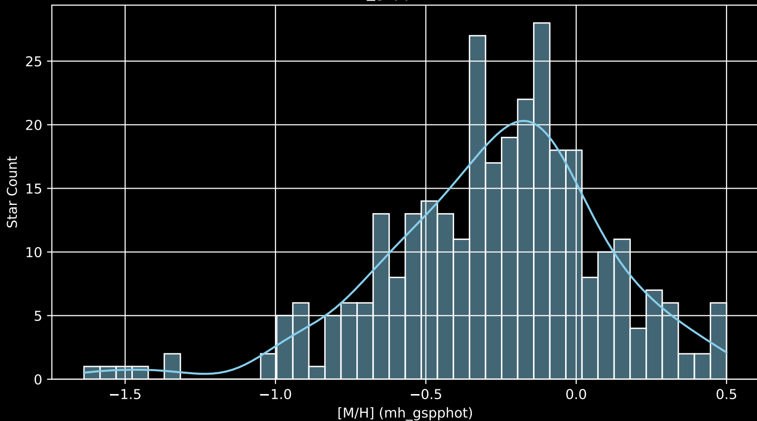
APOGEE DR17 Field: [sgr_tidal10 [M/H] (mh_gspphot) (n= 314)
