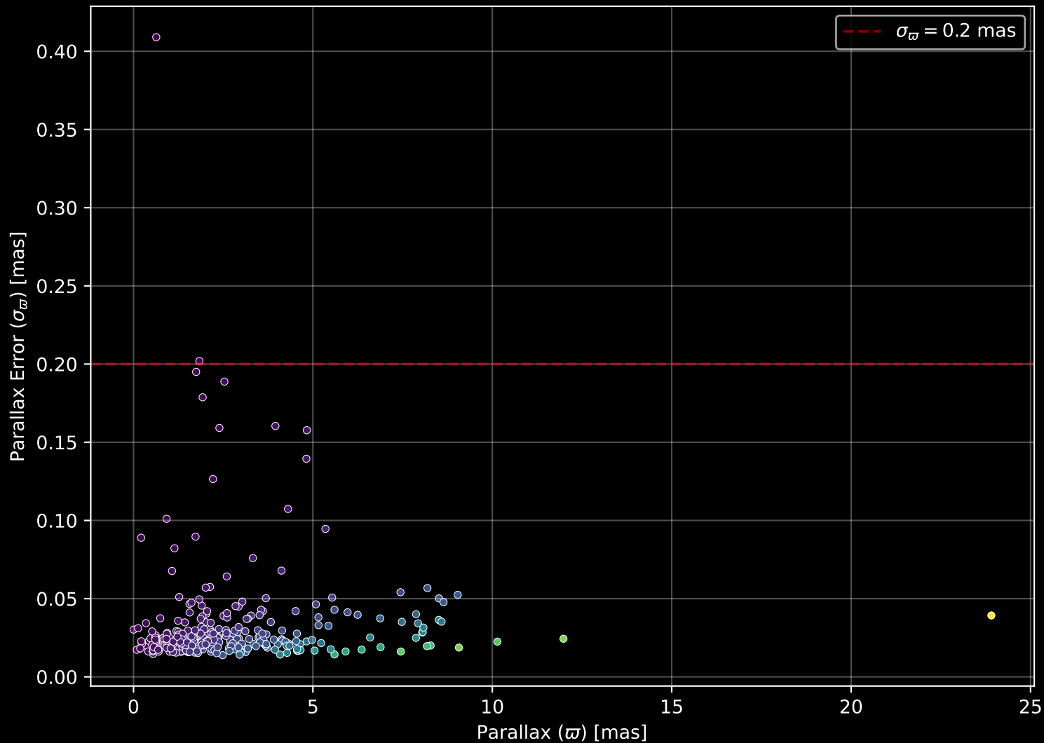
APOGEE DR17 Field: [sgr_tidal10] Parallax Quality (n= 315)
